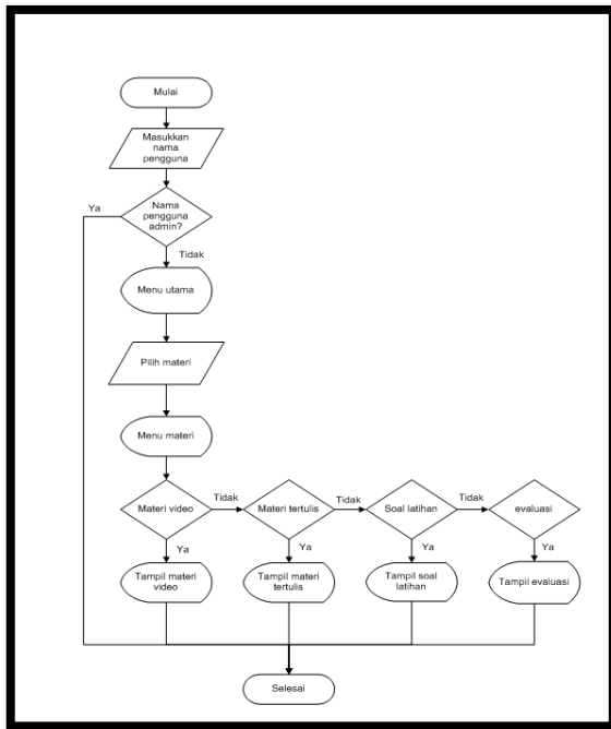
Gambar 4.3 Flowchart sistem user
