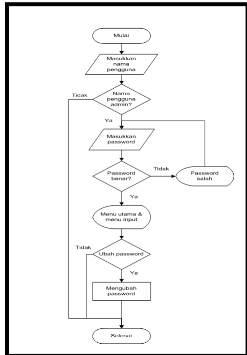
Gambar 4.2 Flowchart sistem admin
