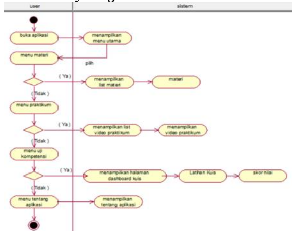
Gambar 3. Activity Diagram Menu Utama
