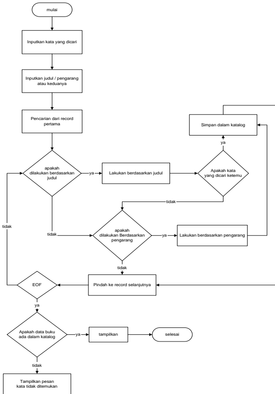
Gambar 3. Flowchart sistem
