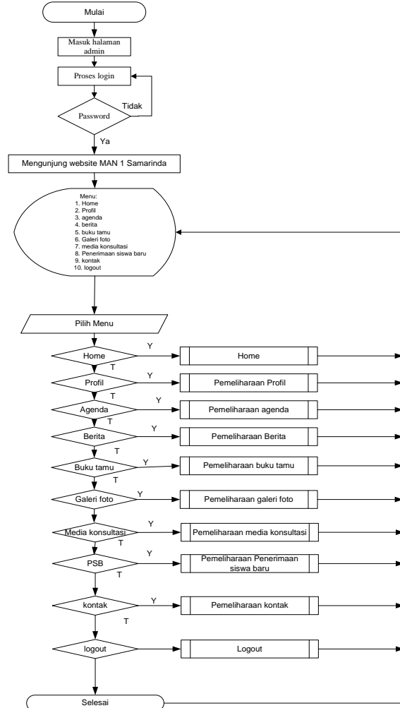
Gambar 3 . flowchart Admin
