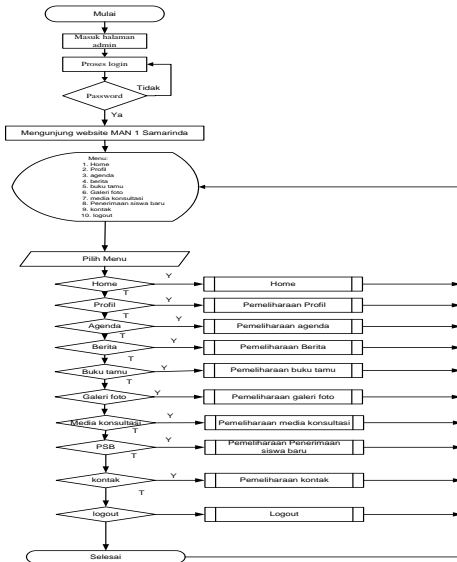
Gambar 1. Flowchart
