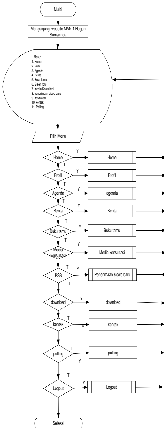
Gambar 4. Flowchart admin
