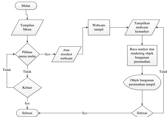
Gambar 4. Flowchart Program
