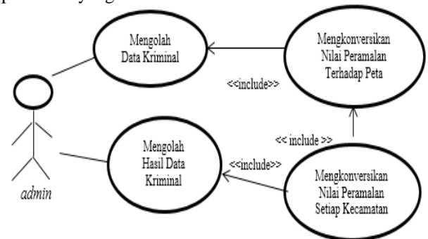
Gambar 3. Use Case Diagram Admin Sistem
