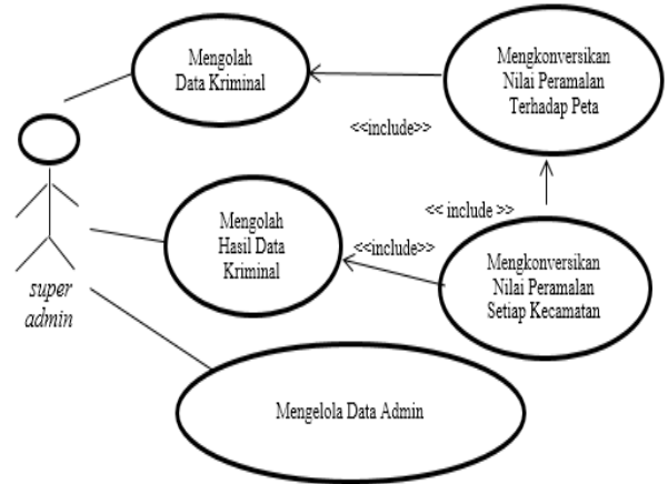
Gambar 2. Use Case Diagram Super Admin Sistem
